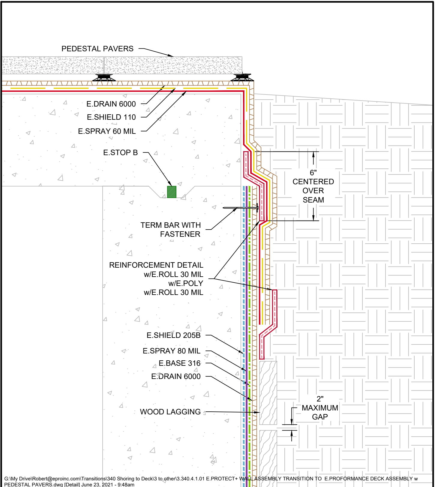
E.PROTECT+ WALL ASSEMBLY - WOOD LAGGING - TRANSITION TO E.PROFORMANCE DECK ASSEMBLY w/PEDESTAL PAVERS
