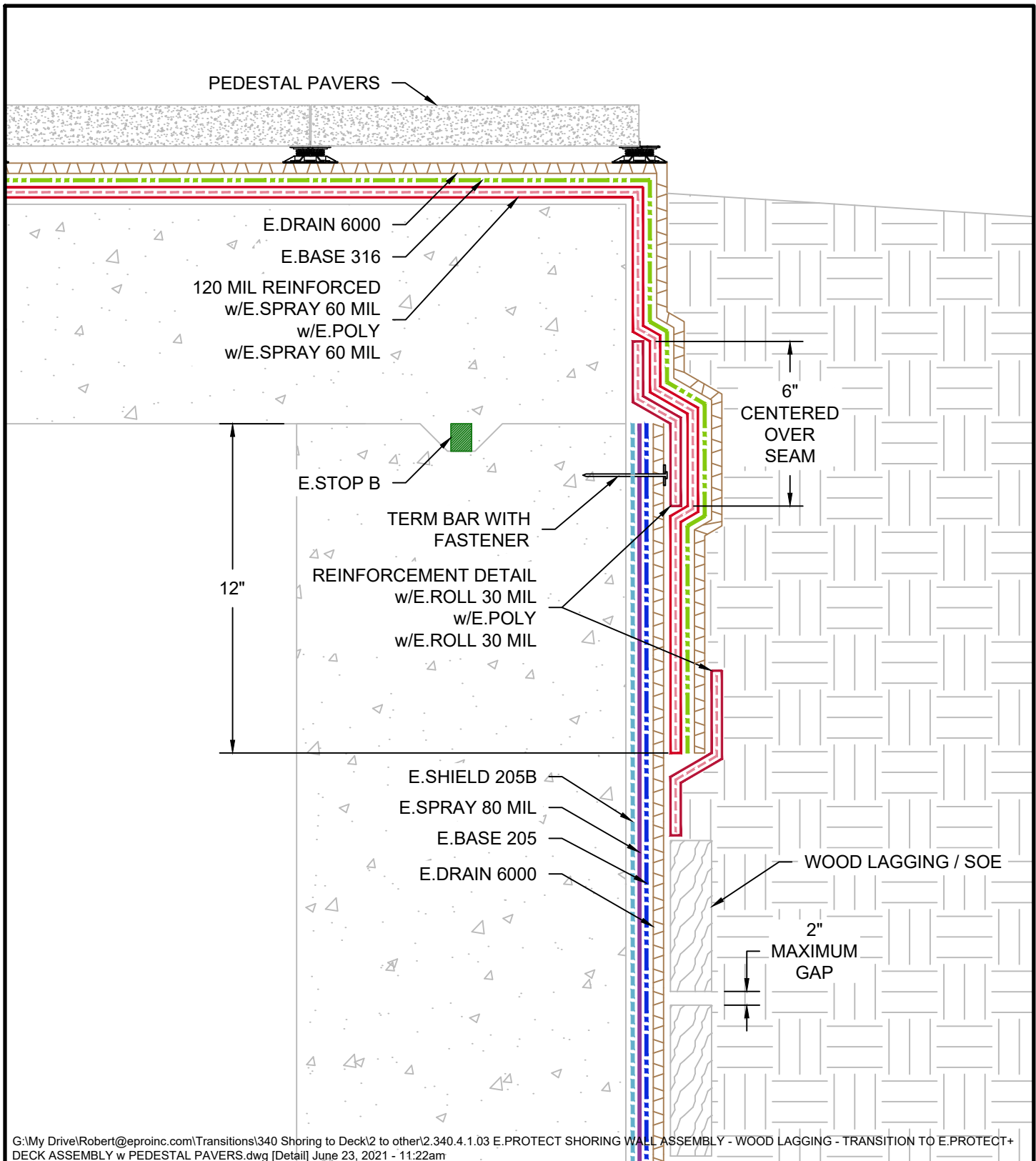
E.PROTECT SHORING WALL ASSEMBLY - WOOD LAGGING - TRANSITION TO E.PROTECT+ DECK ASSEMBLY w PEDESTAL PAVERS
