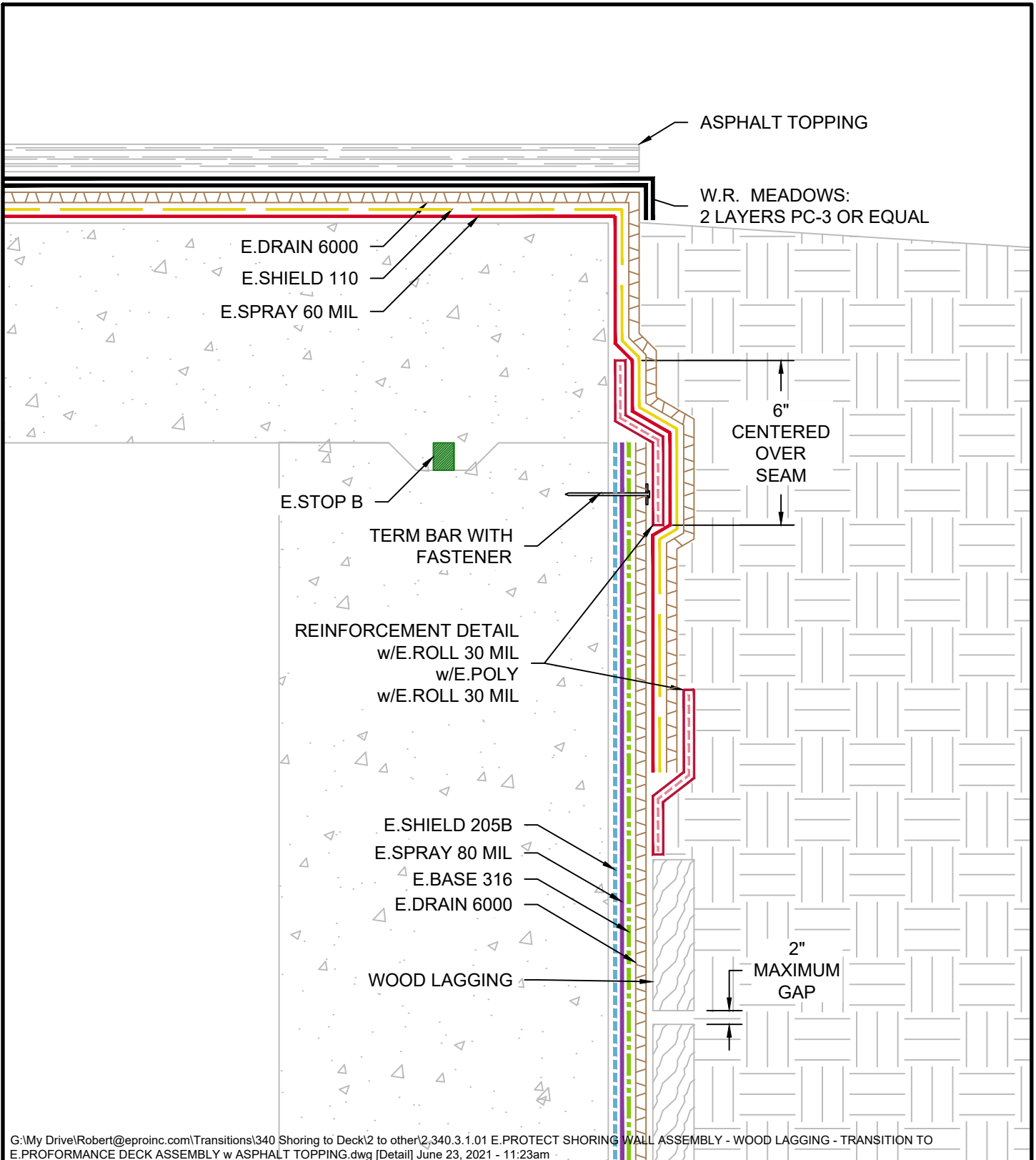
E.PROTECT SHORING WALL ASSEMBLY - WOOD LAGGING - TRANSITION TO E.PROFORMANCE DECK ASSEMBLY with ASPHALT TOPPING
