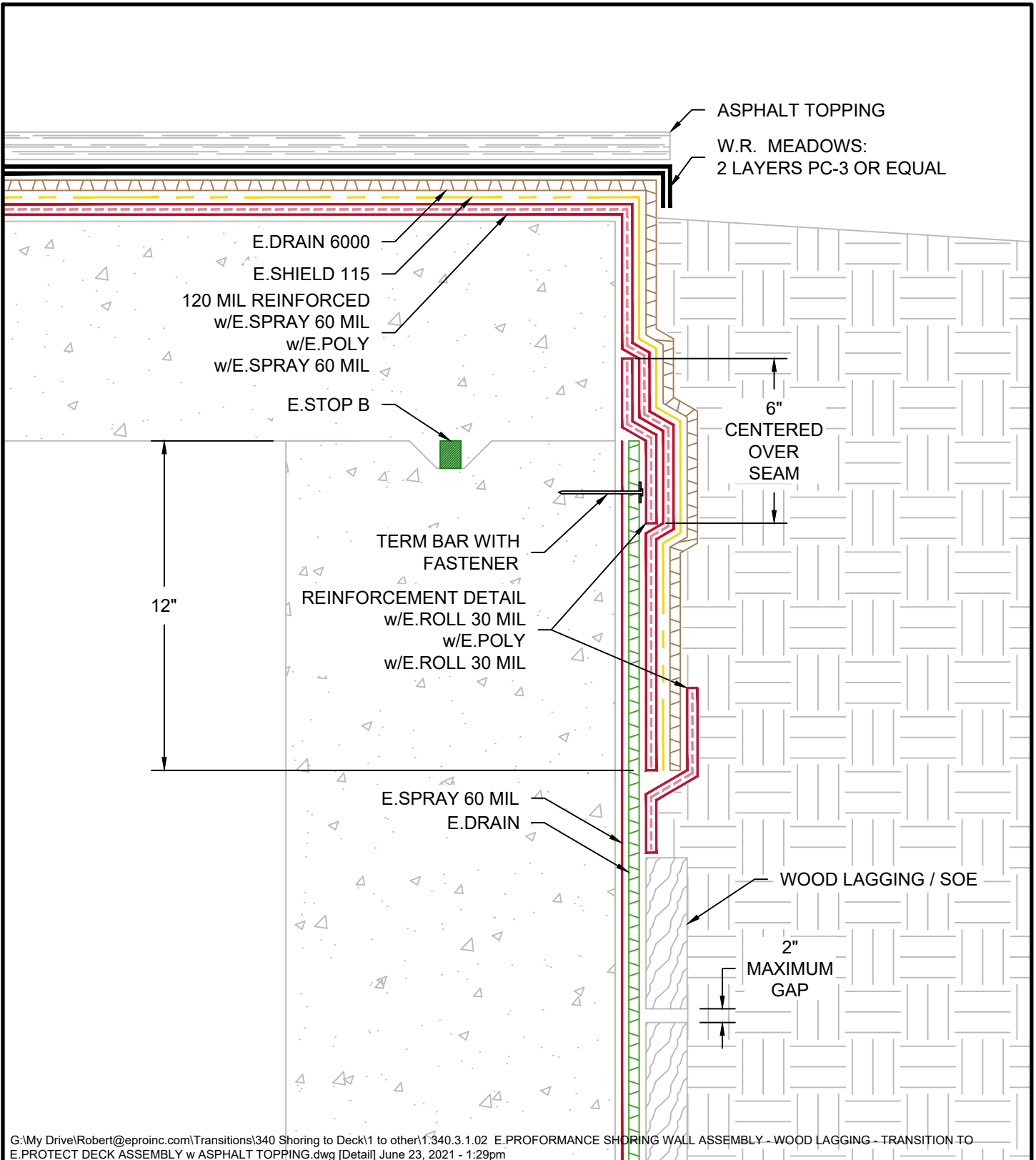
E.PROFORMANCE SHORING WALL ASSEMBLY - WOOD LAGGING - TRANSITION TO E.PROTECT DECK ASSEMBLY w ASPHALT TOPPING
